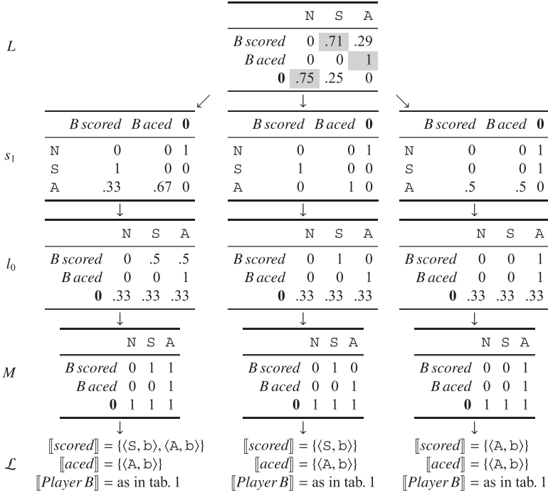
Figure 2 Simple scalar inference. We assume a flat prior over states and lexica. C(\mathbf{0}) = 5 , and C(m) = 0 for the other messages. The uncertainty listener L infers that the general term scored excludes its specific counterpart aced in this context.
