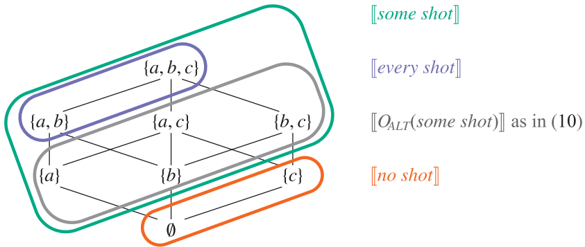
Figure 1 Given a domain \{a,b,c\} with \llbracket shot \rrbracket = \{a,b\} , \llbracket some\ shot \rrbracket is equal to the set of sets in the green box, \llbracket every\ shot \rrbracket to the set of sets in the purple box, and \llbracket no\ shot \rrbracket to the set of sets in the orange box. If ALT(some\ shot) contains \llbracket every\ shot \rrbracket , then some\ shot is refined to exclude the purple subset.
